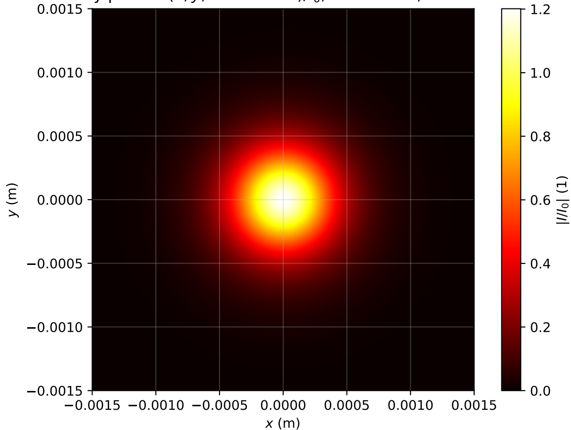
Intensity profile I(x, y, z = 1.433m)/I_0 , \text{Pin}=0.7\text{Pcr} , artificial time
